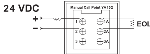
Diagram for Fire Alarm System, 24 VDC
